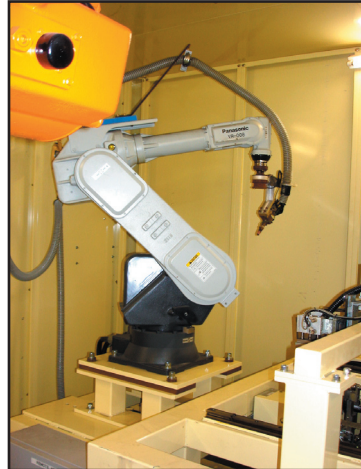
"2003" Panasonic 6 Axis Model VR-008 GII Robotic Welding Cell
