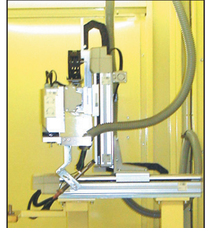
"2003" Panasonic 3 Axis Model ISP Cartesian Robotic Tig Welding Cell
